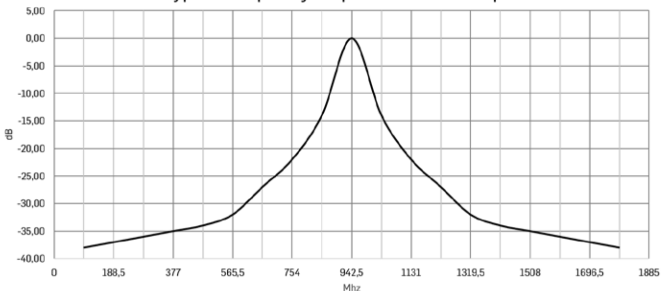
Typical frequency response for EP-33A probe
